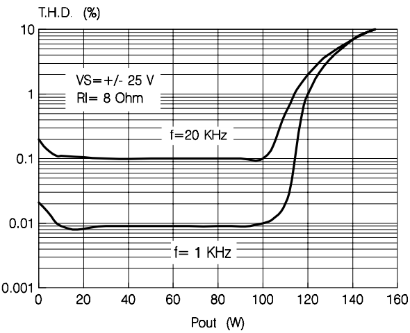
Figure 27: Distortion vs. Output Power
