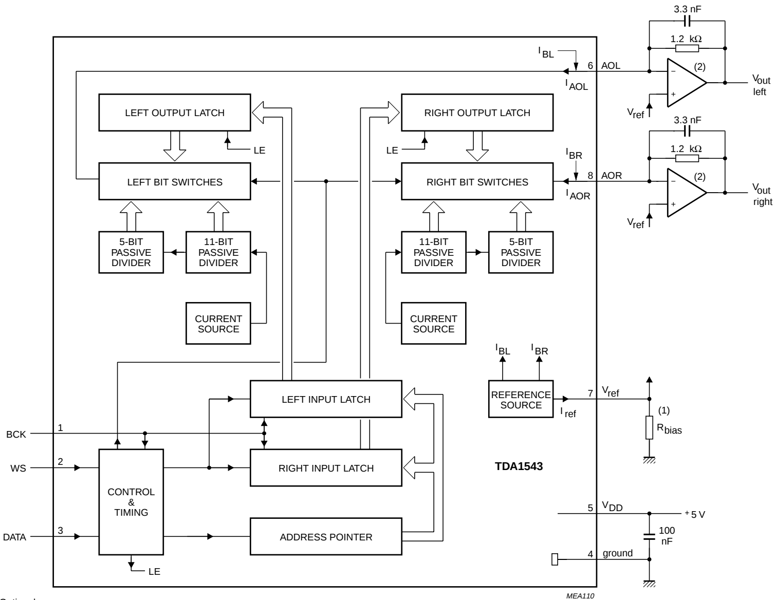
Fig.1 Block diagram.
