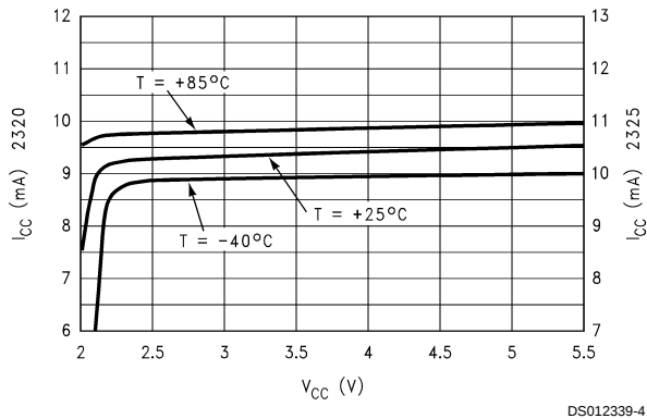
I_{CC} vs V_{CC} LMX2320/25
