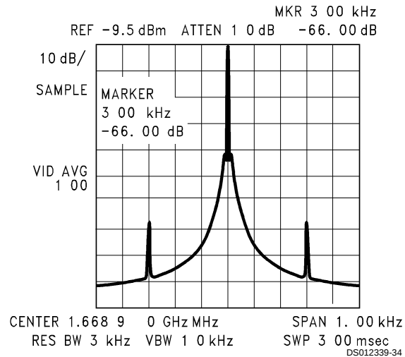
FIGURE 10. PLL Reference Spurs
