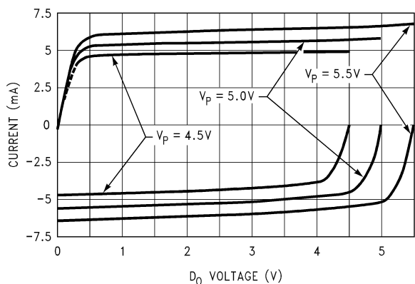
Charge Pump Current vs D_0 Voltage
