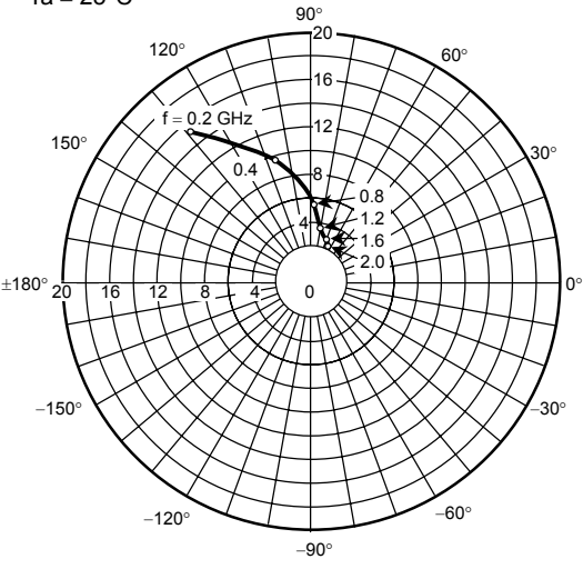
S 21e V CE = 5 V I C = 10 mA T a = 25°C
